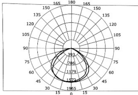
Luminous Intensity Distribution Curve
